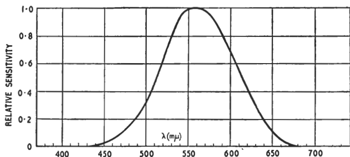
Fig. 1.7. Response of the eye
