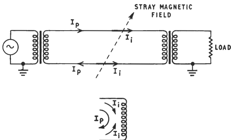
Fig. 1.31. Example of a balance/unbalance connection
