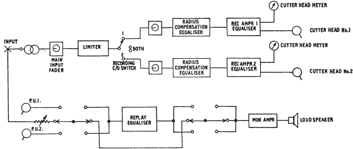
Fig. 2.38. Schematic diagram of a twin-machine recording channel
