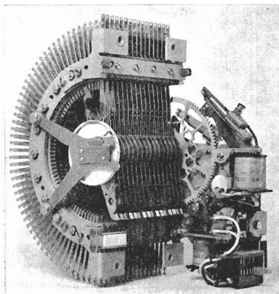
Fig. 2.22. Motorised unselector switch (by courtesy of Associated Electrical Industries)
