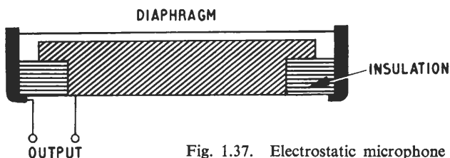
Fig. 1.37. Electrostatic microphone
