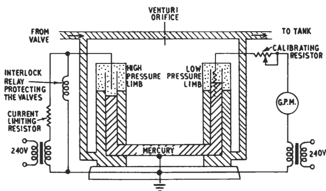
Fig. 5.19. The Electroflo body
