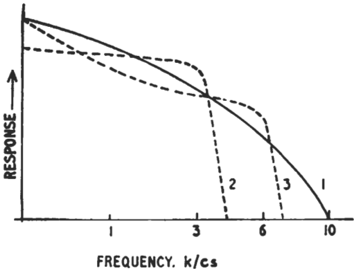
Fig. 6.10. The effect of loading on line-frequency response
