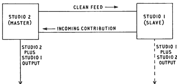
Fig. 2.15. Operation of a clean-feed system
