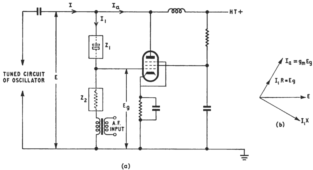
Fig. 5.23. A reactance valve circuit
