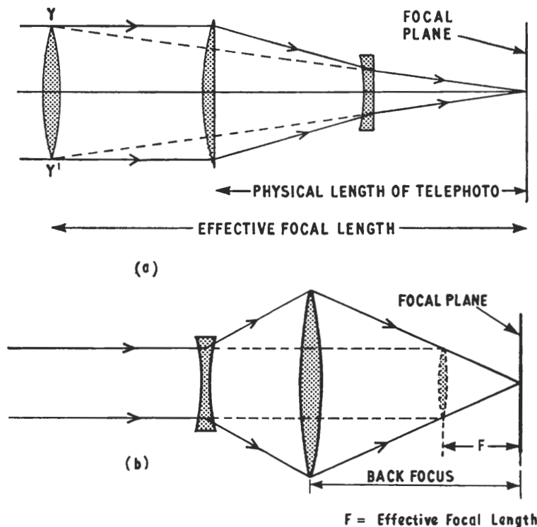
Fig. 1.12. (a) telephoto lens; (b) reverse telephoto lens
