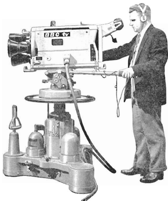
Fig. 3.6. The pedestal dolly
