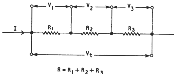
Fig. 1.14. Resistances in series
