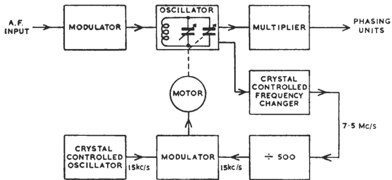
Fig. 5.24. Schematic diagram of the mean frequency control circuit for an LC oscillator f.m. drive
