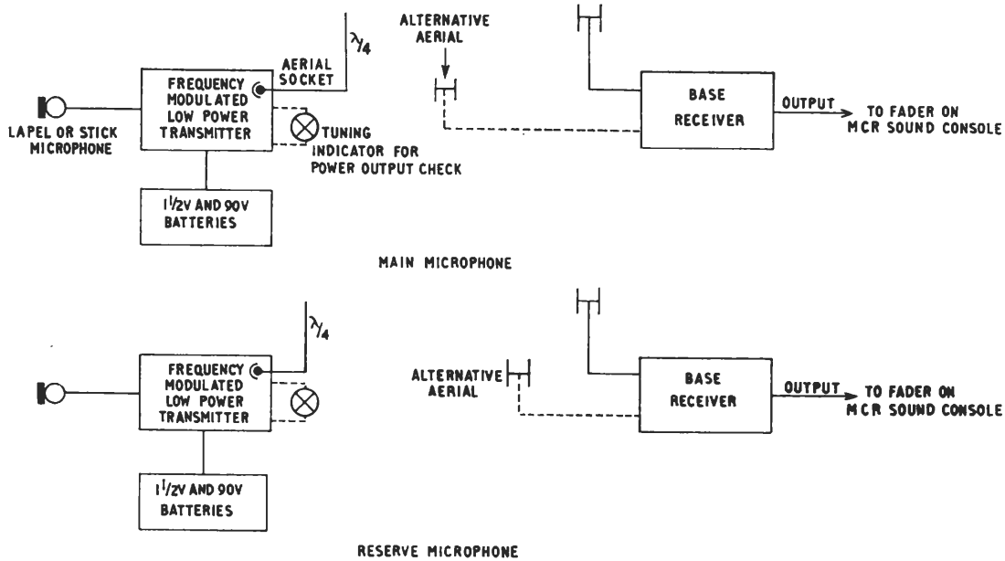
Fig. 4.9. Schematic diagram of the radio microphone
