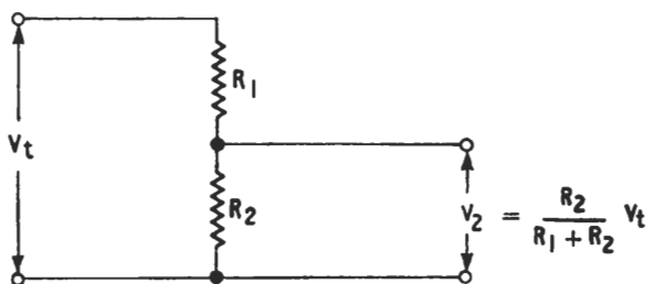
Fig. 1.16. Voltage division
