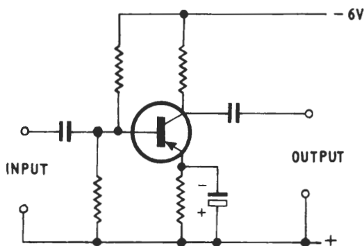
Fig. 1.52. Transistor amplifier
