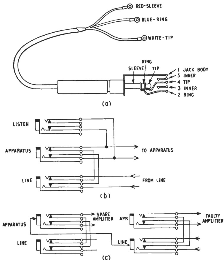
Fig. 2.21. (a) Plug and jack connections; (b) jack connections providing listen, apparatus and line facilities
