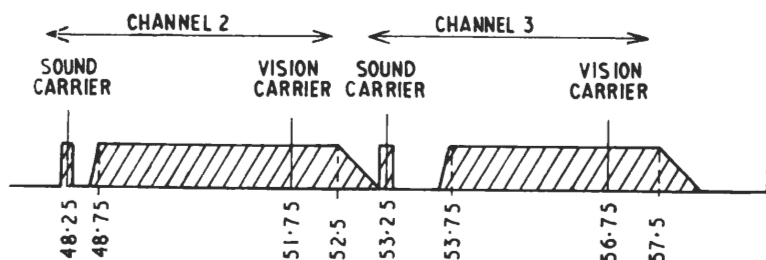
Fig. 5.27. The frequency ranges in Mc/s for the television and sound transmitters in channels 2 and 3
