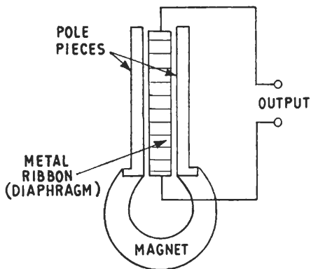
Fig. 1.36. Ribbon microphone
