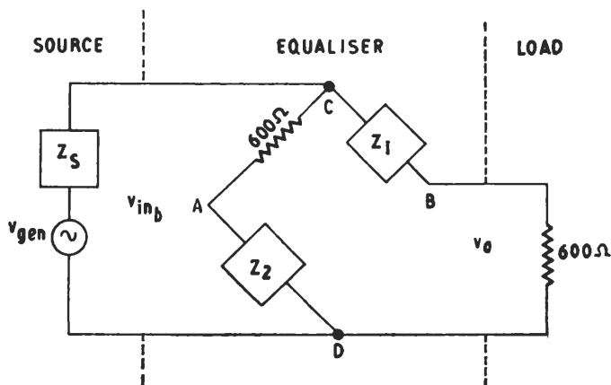
Fig. 6.16. The constant-resistance bridge-type equaliser
