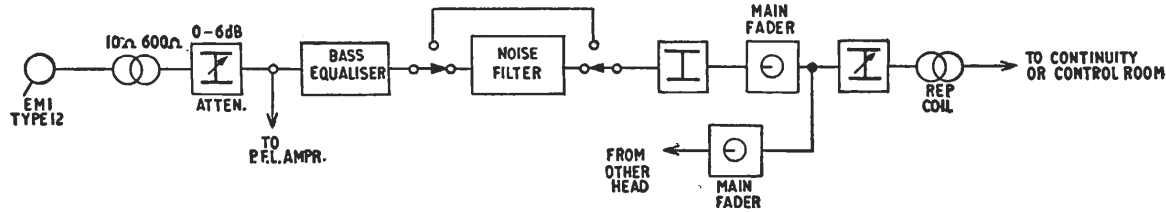
Fig. 2.45. Programme circuits of the TD/7 reproducing desk
