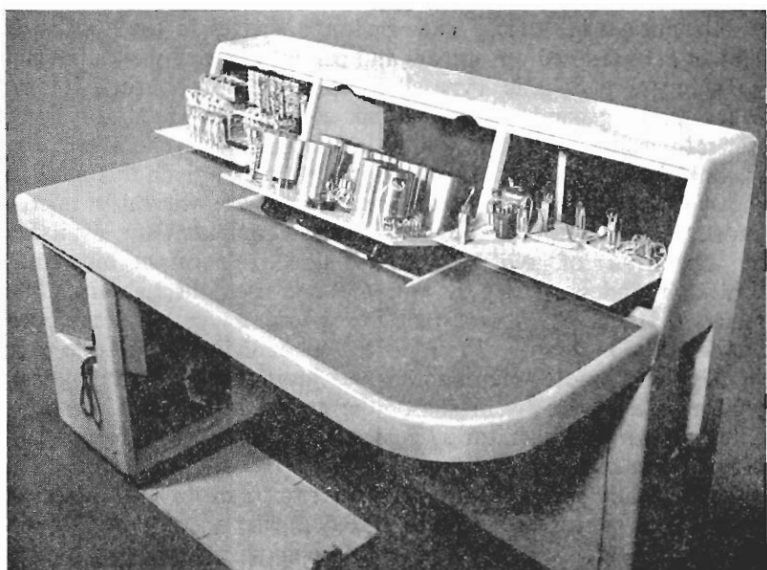
Fig. 2.11. Studio control desk Type A, Mark V. The top photograph shows a general view of the control desk and the lower photograph shows the panels swung forward for inspection and maintenance with the side panel of the pedestal removed
