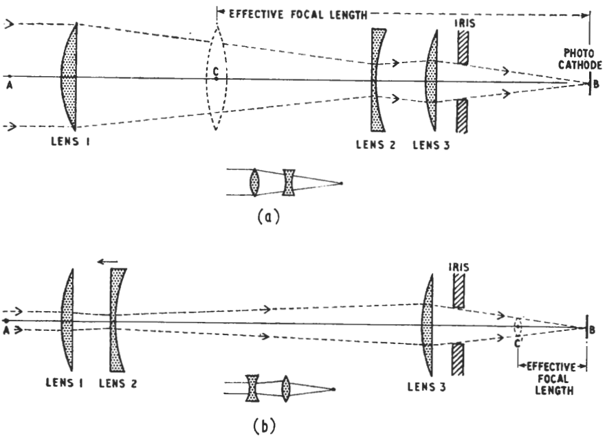
Fig. 4.5. The zoom lens
