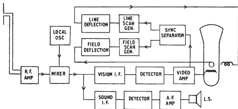
Fig. 1.66. Schematic diagram of a television receiver
