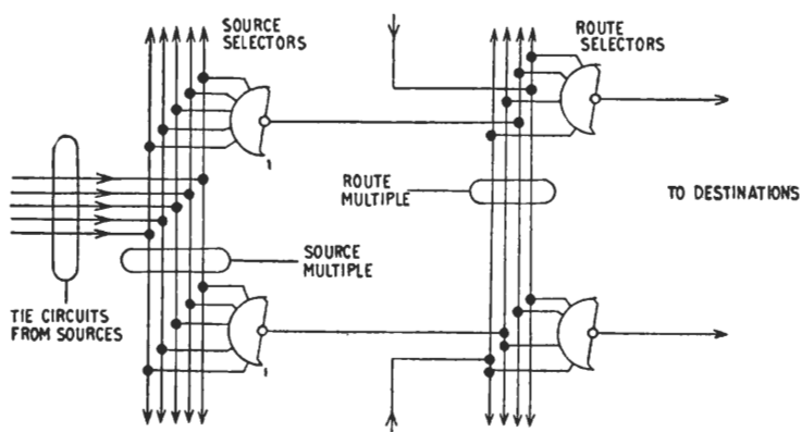
Fig. 2.23. Source and route selection by unselector
