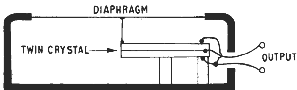
Fig. 1.38. Crystal microphone
