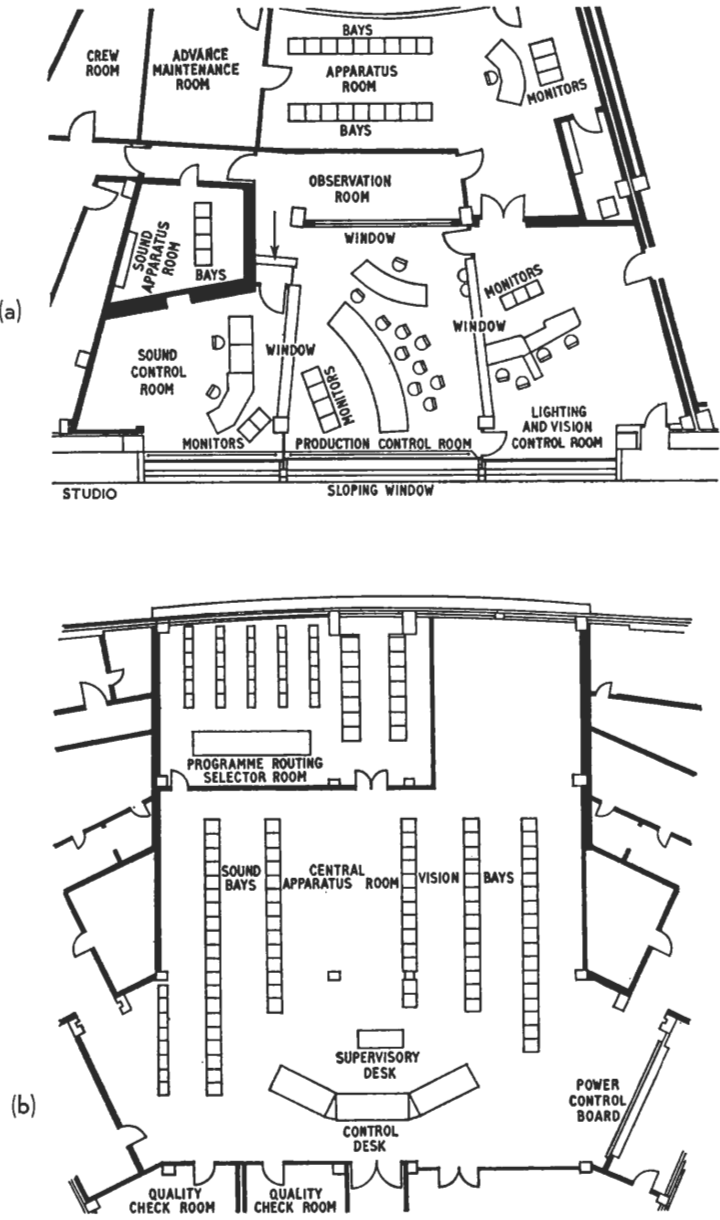
Fig. 3.2. (a) Plan view of a typical studio at television centre; (b) Plan view of the central apparatus room at television centre
