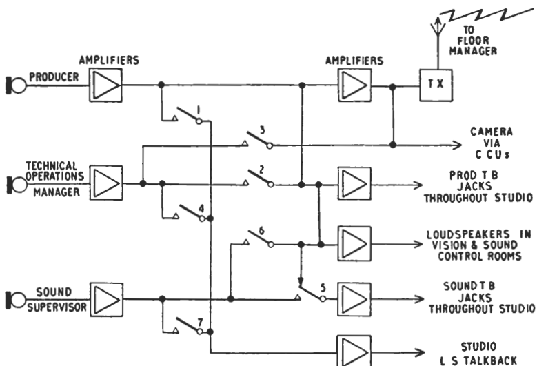
Fig. 3.27. Simplified diagram of the talk-back system
