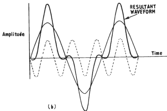
Fig. 1.54. (a) fundamental with a 3rd harmonic starting in phase; (b) fundamental with a 3rd harmonic starting out of phase
