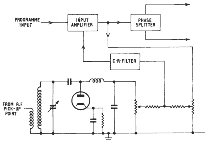
Fig. 5.34. The reduction of hum and noise in the sound transmitter by using negative feedback
