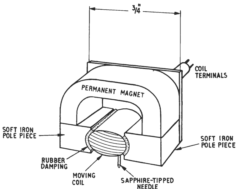
Fig. 2.42. Moving-coil replay head
