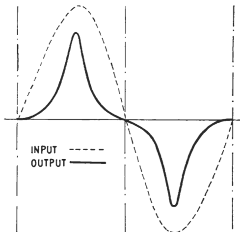
Fig. 2.31. Reproduced waveshape when a sinusoidal tone input is applied alone to the recording head
