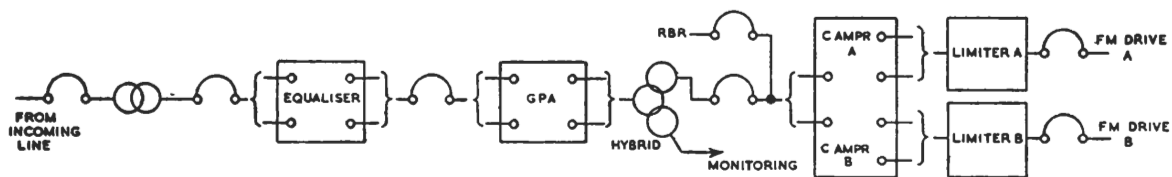
Fig. 5.25. Schematic diagram of the programme input equipment for an f.m. transmitter
