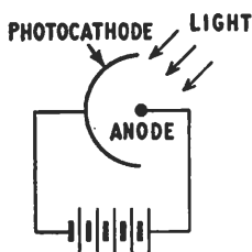
Fig. 1.39. Photo-electric cell
