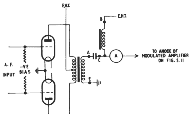
Fig. 5.12. A Class B push-pull modulator stage
