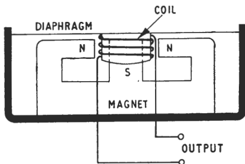
Fig. 1.35. Moving-coil microphone
